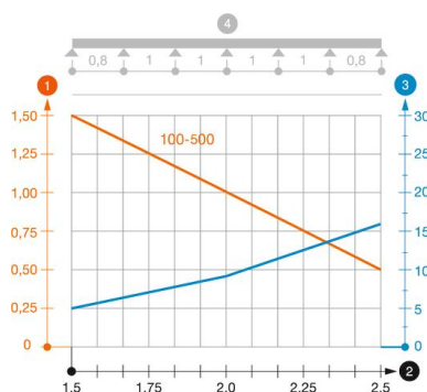
Load diagram, cable tray, type GKS FL60
